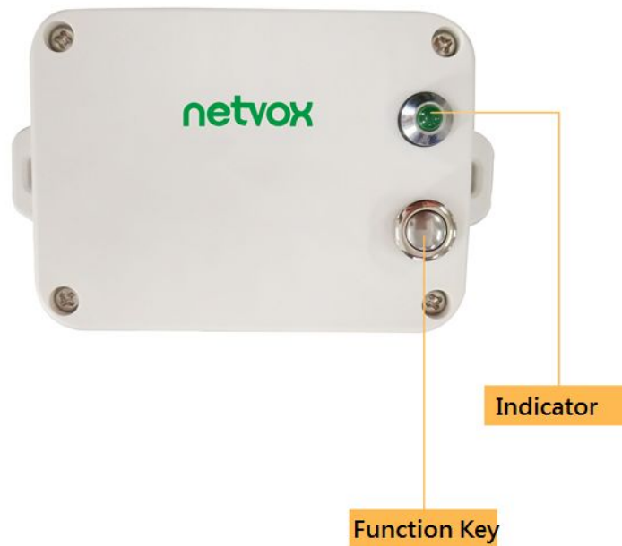
Fig.1 R718MBC Appearance
